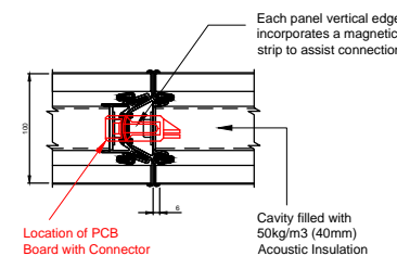
Type "U" Protective Vertical Frame
