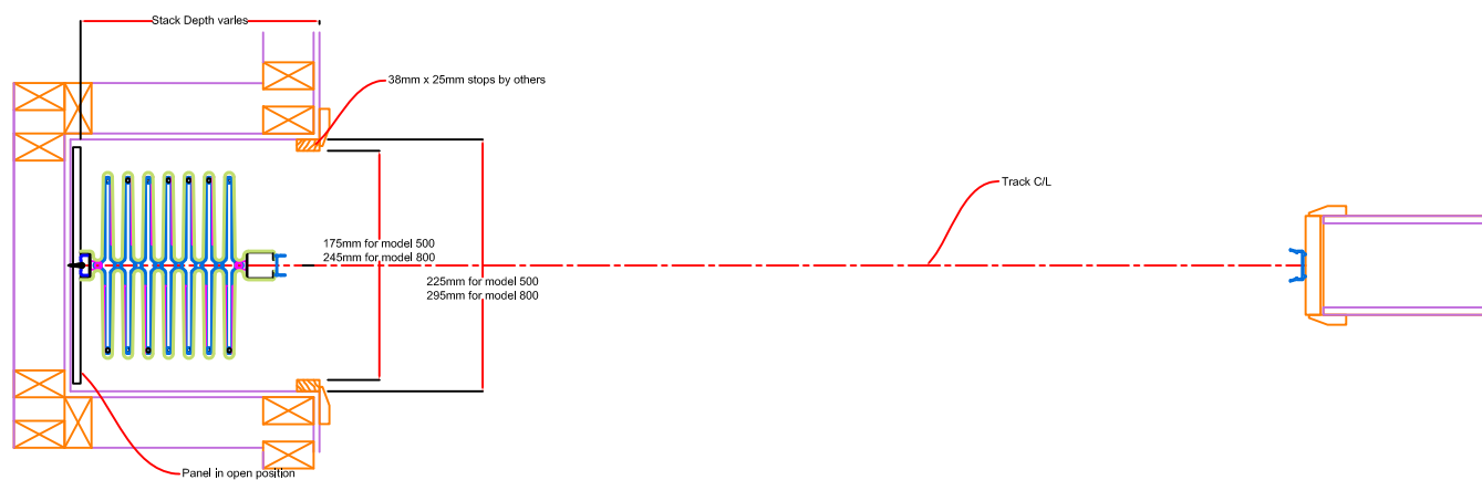
SLIDING DOOR PANEL IN POCKET
